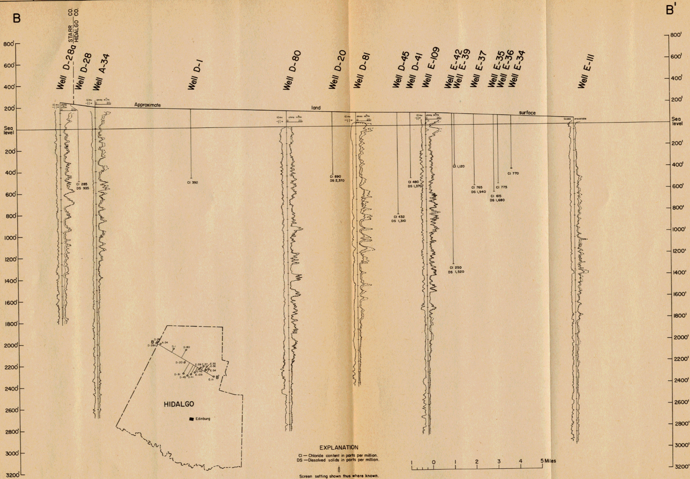
GEOLOGIC SECTION B-B', HIDALGO COUNTY, TEXAS
